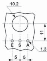
viewed on component side
