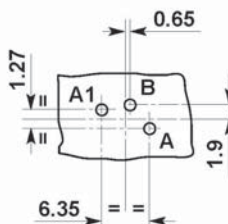
viewed on component side
