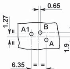
ST 1044 1-pole
