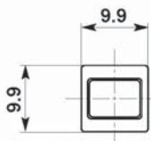
ST 1044 1-pole
