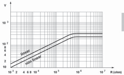
Max working voltage curve
