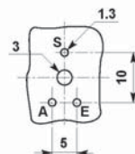
viewed on component side
