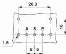
viewed on component side
